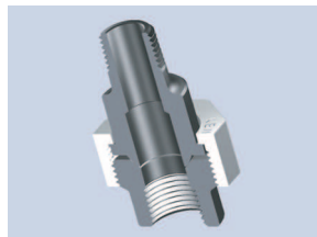
3000# "AAR" Unions Steel-to-Steel Threaded Male X Female
