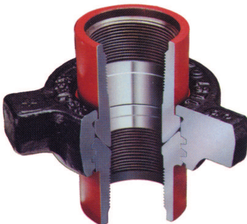
FIGURE 400 BLACK NUT, RED SUBS
